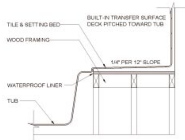
BUILT-IN TRANSFER SEAT DETAIL
