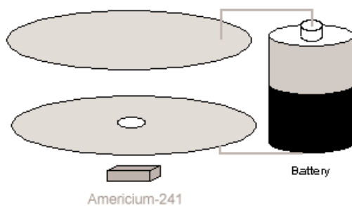
IONIZATION SMOKE DETECTOR COMPONENTS
