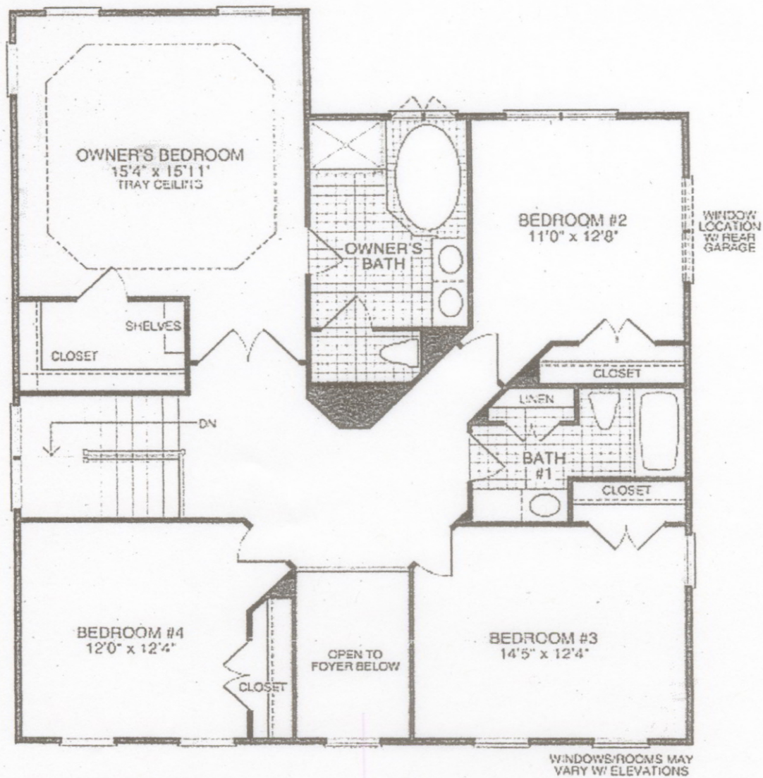
Second Floor Plan Elevation B
